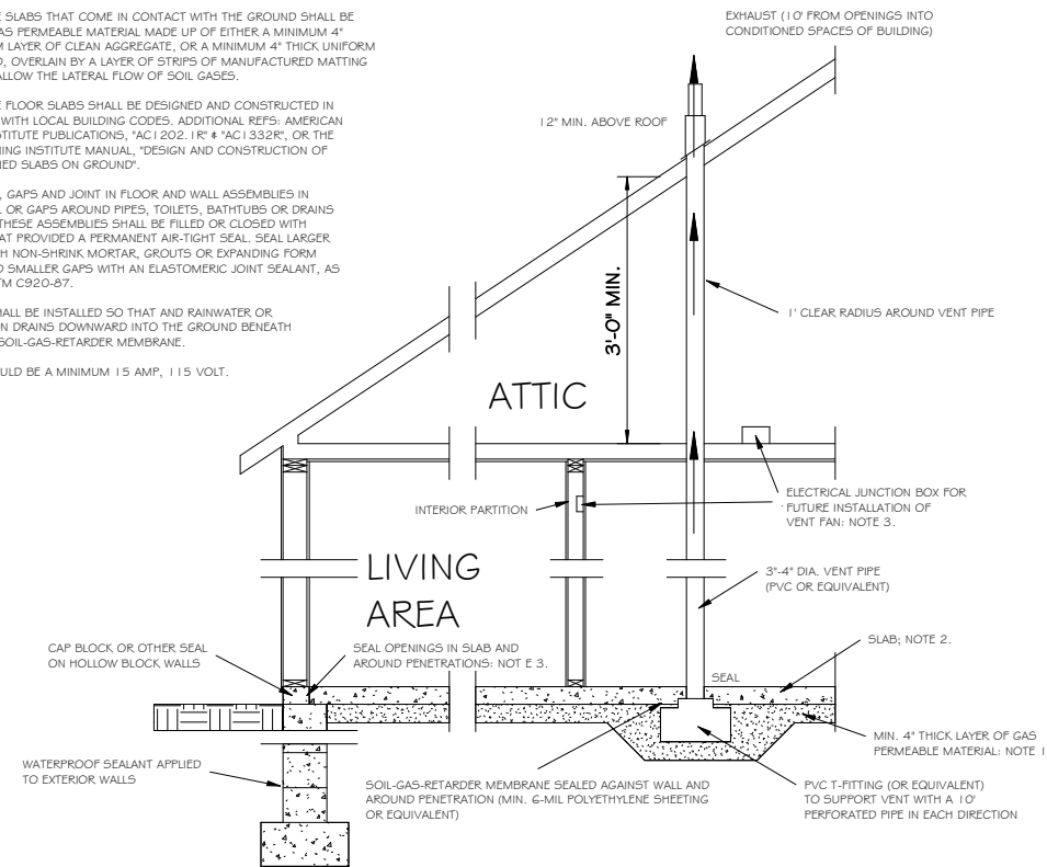
3 - Radon Section 1/2" = 1'-0"
