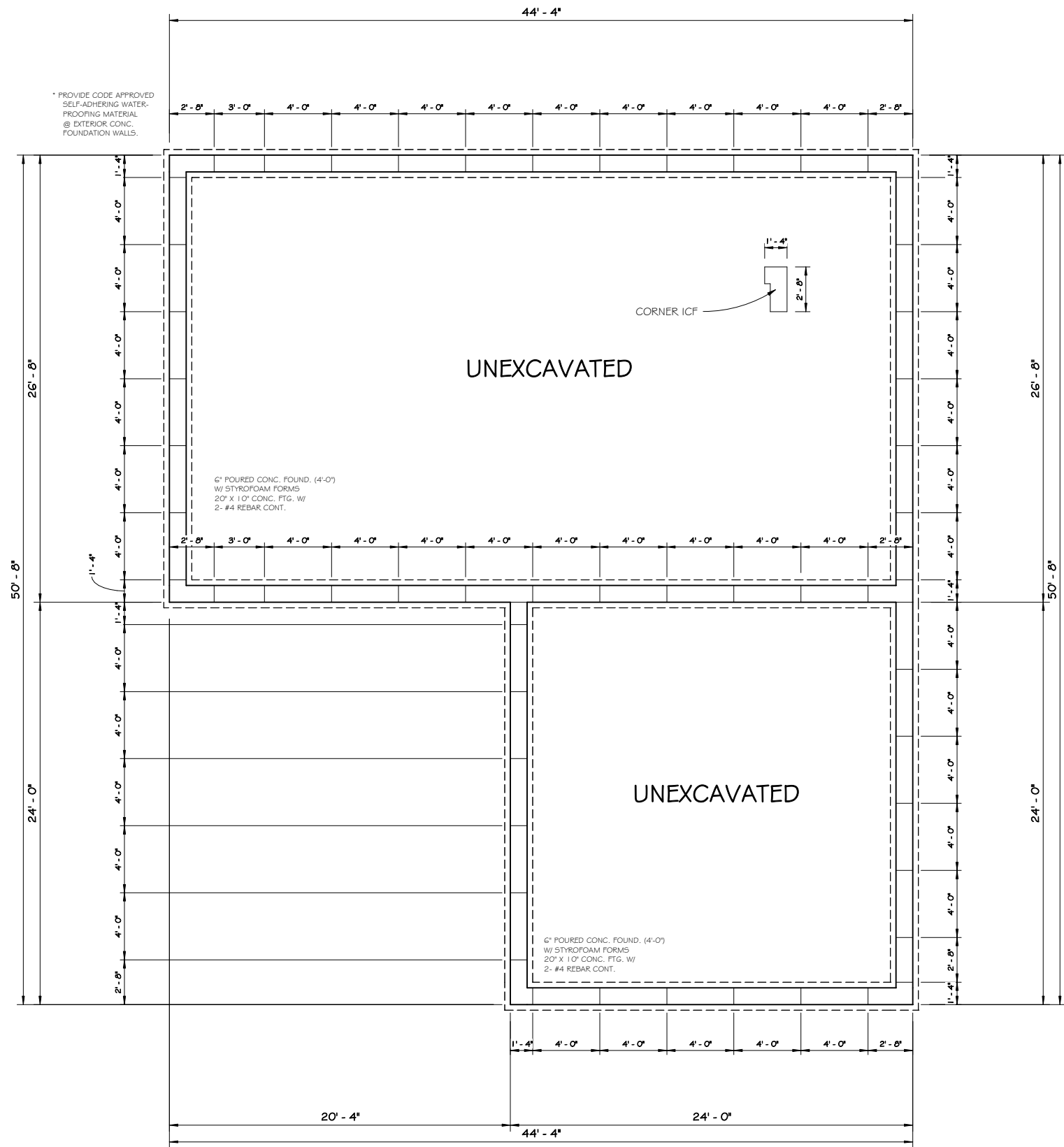
1 BASEMENT PLAN 1/4" = 1'-0"
