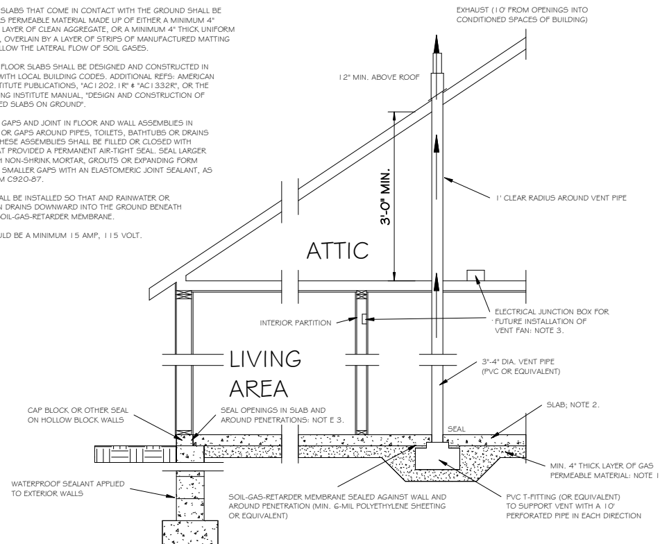
3 - Radon Section 1/2" = 1'-0"
