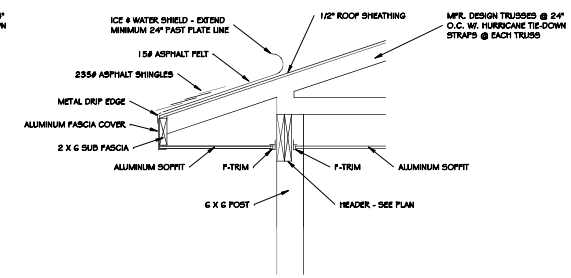
4 ROOF DETAIL 1" = 1'-0"
