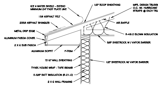
4 ROOF DETAIL 1" = 1'-0"
