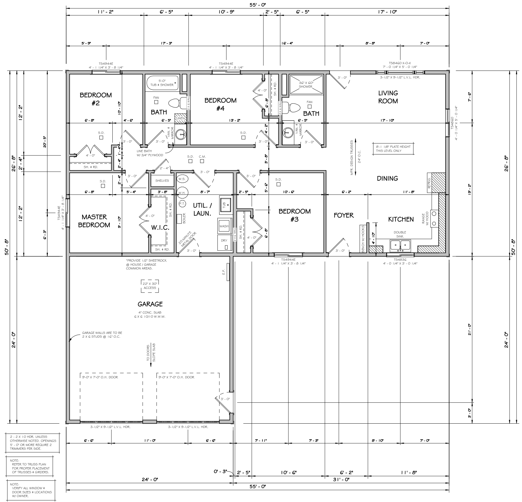
1 MAIN LEVEL 1/4" = 1'-0"
