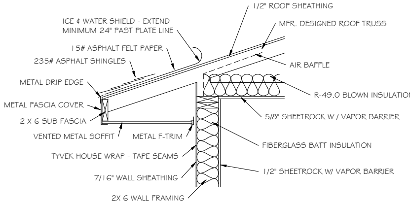
3 - Roof Details 1" = 1'-0"
