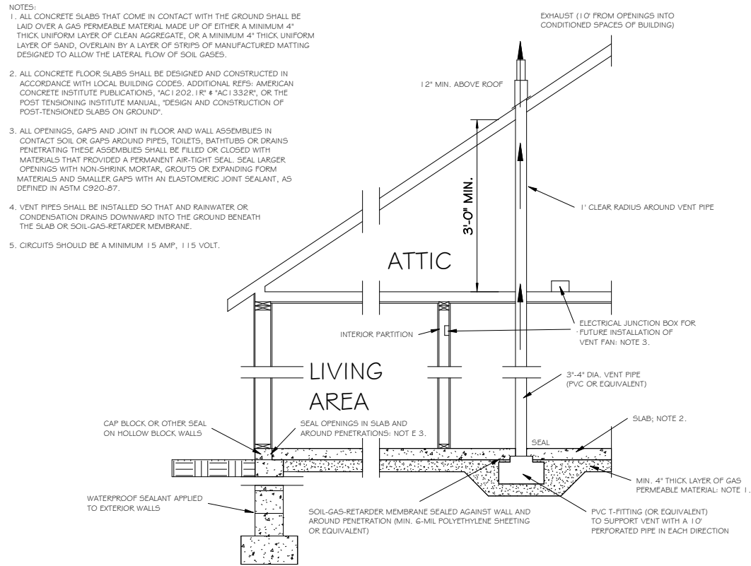
2 - Radon Section 1/2" = 1'-0"
