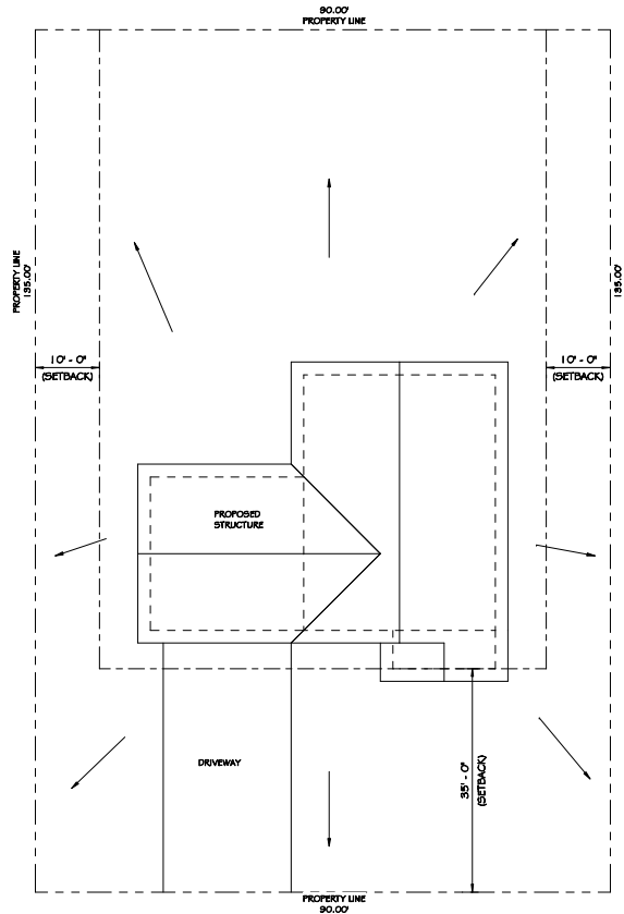
SITE PLAN 1" = 10'-0"
