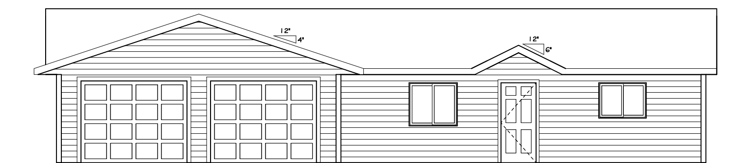
4 FRONT 1/4" = 1'-0"
