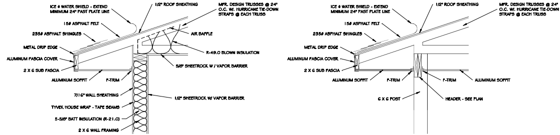
4 ROOF DETAIL 1" = 1'-0"
