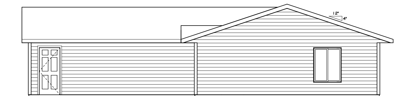
2 RIGHT 1/4" = 1'-0"
