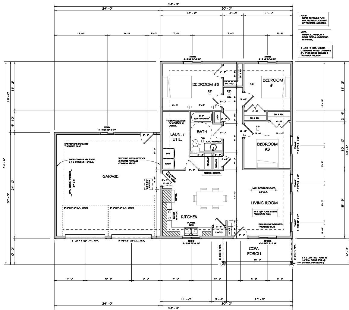
1 MAIN LEVEL AS 1/4" = 1'-0"
