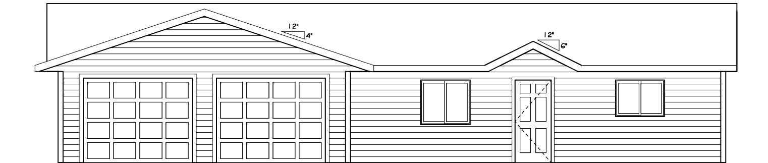
4 FRONT AI 1/4" = 1'-0"
