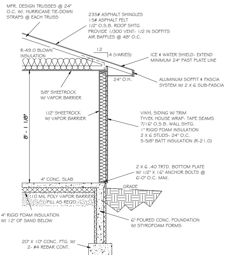
6 - Wall Section AI 1/2" = 1'-0"
