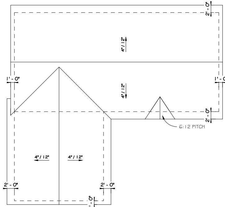
5 ROOF PLAN AI 1/8" = 1'-0"
