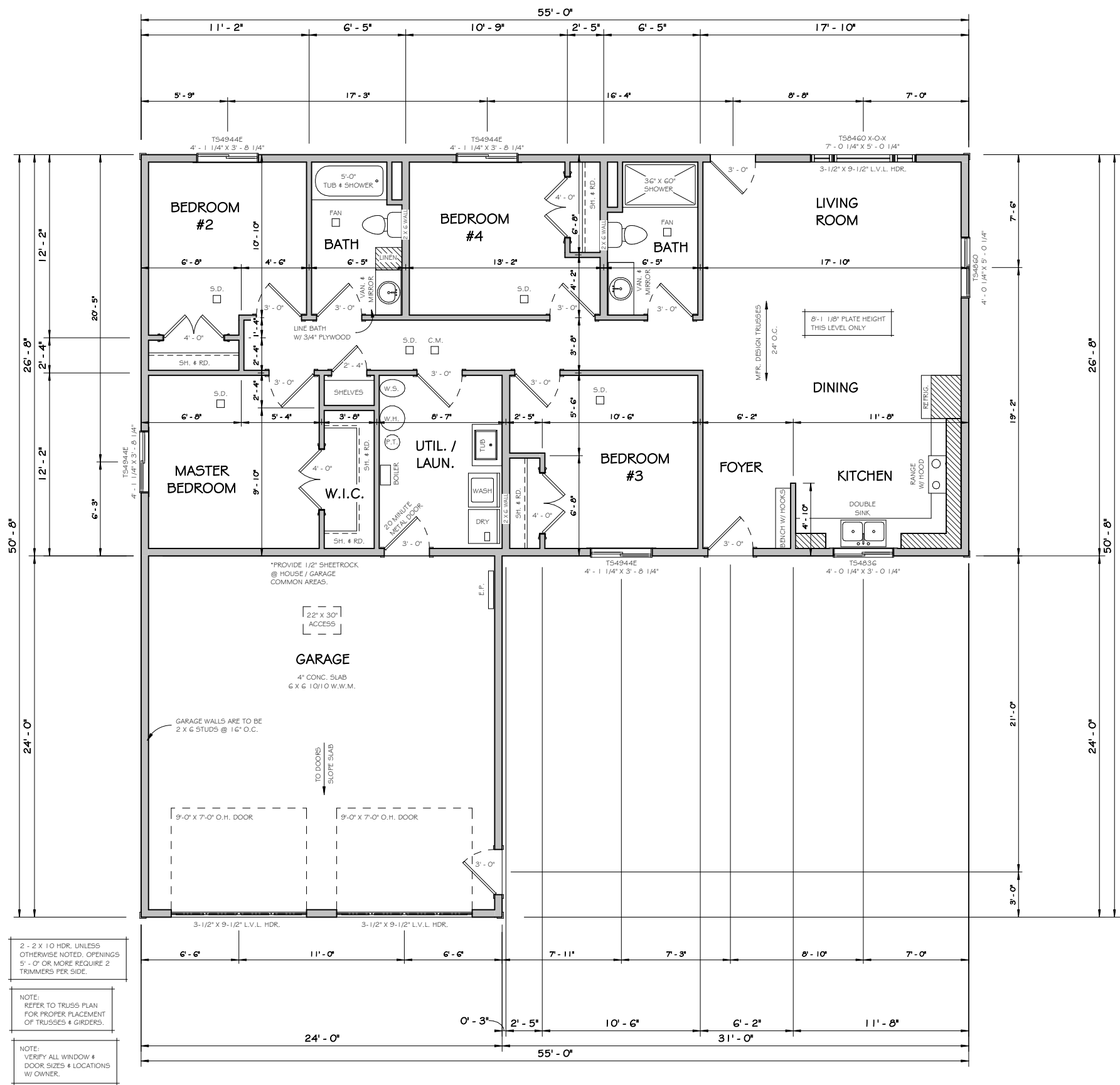
1 MAIN LEVEL 1/4" = 1'-0"
