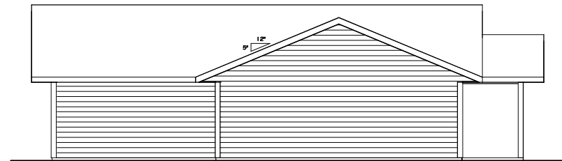
2 LEFT ELEVATION 1/4" = 1'-0"
