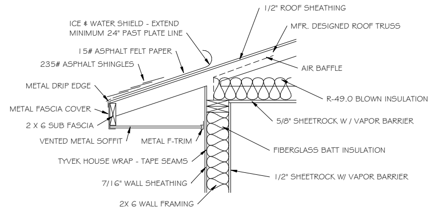
3 - Roof Details 1" = 1'-0"
