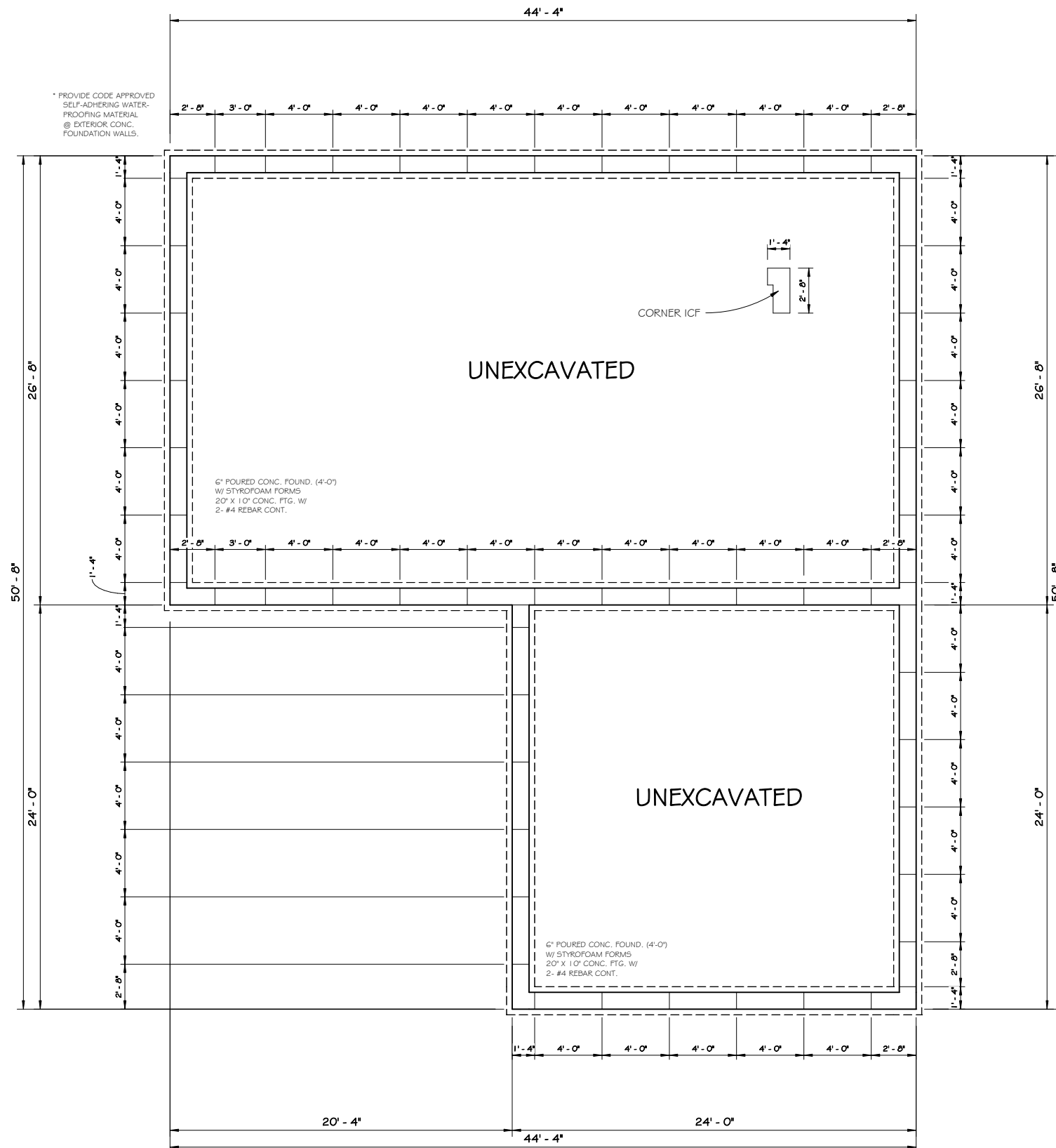
1 BASEMENT PLAN 1/4" = 1'-0"
