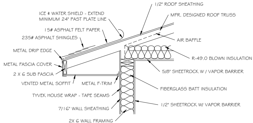
3 - Roof Details 1" = 1'-0"
