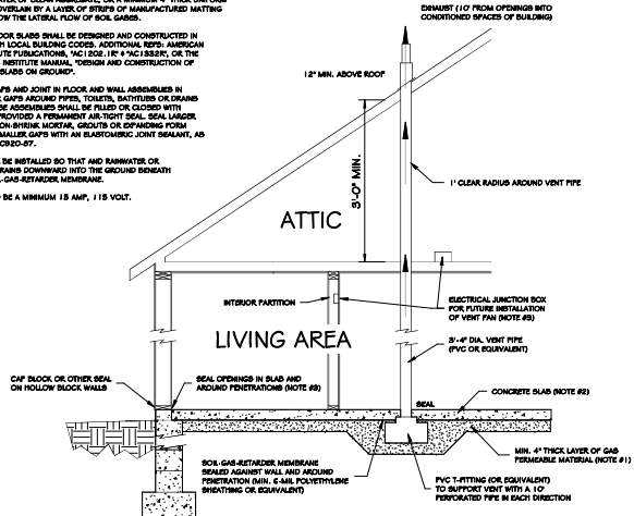
3 RADON SECTION 1/2" = 1'-0"
