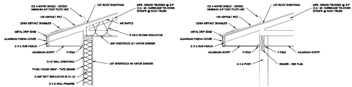
4 ROOF DETAIL 1" = 1'-0"
