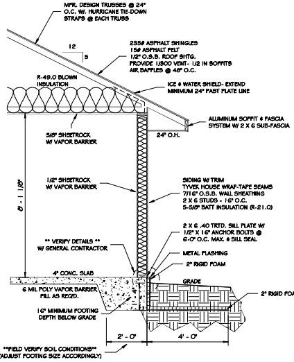
2 WALL SECTION 1/2" = 1'-0"
