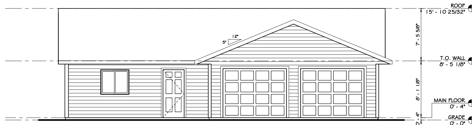
4 FRONT AI 1/4" = 1'-0"
