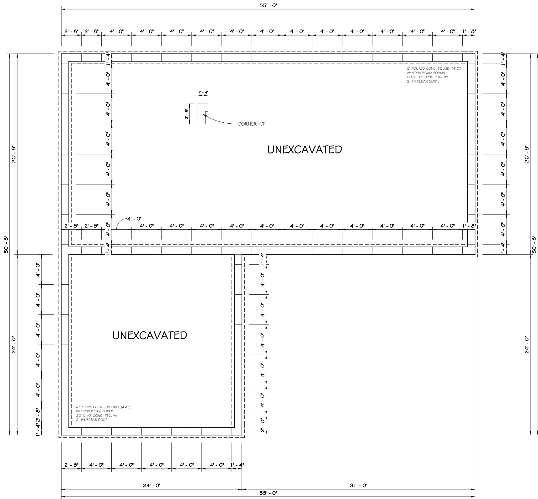
1 BASEMENT PLAN 1/4" = 1'-0"
