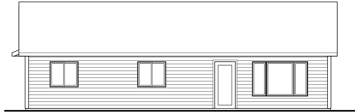
1 REAR AI 1/4" = 1'-0"
