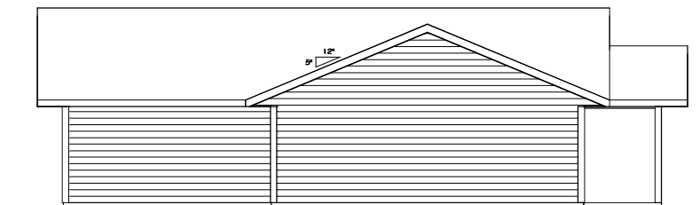
2 LEFT ELEVATION 1/4" = 1'-0"
