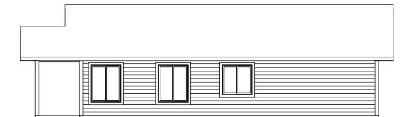
3 RIGHT ELEVATION 1/4" = 1'-0"
