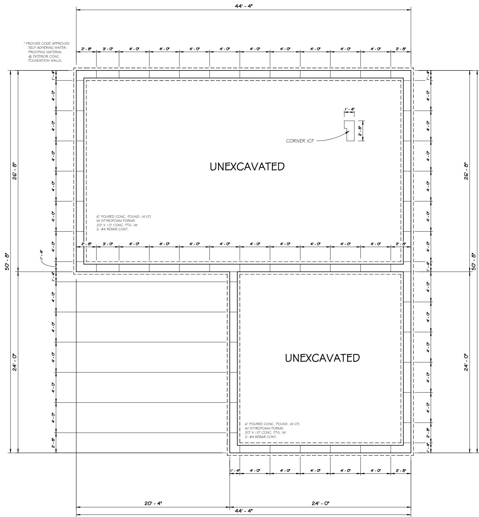
1 BASEMENT PLAN 1/4" = 1'-0"
