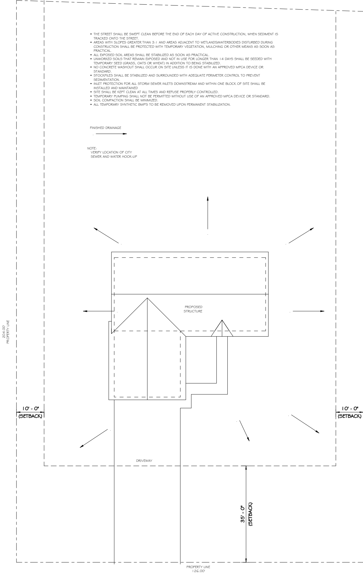
2 SITE PLAN A2 3/32" = 1'-0"
