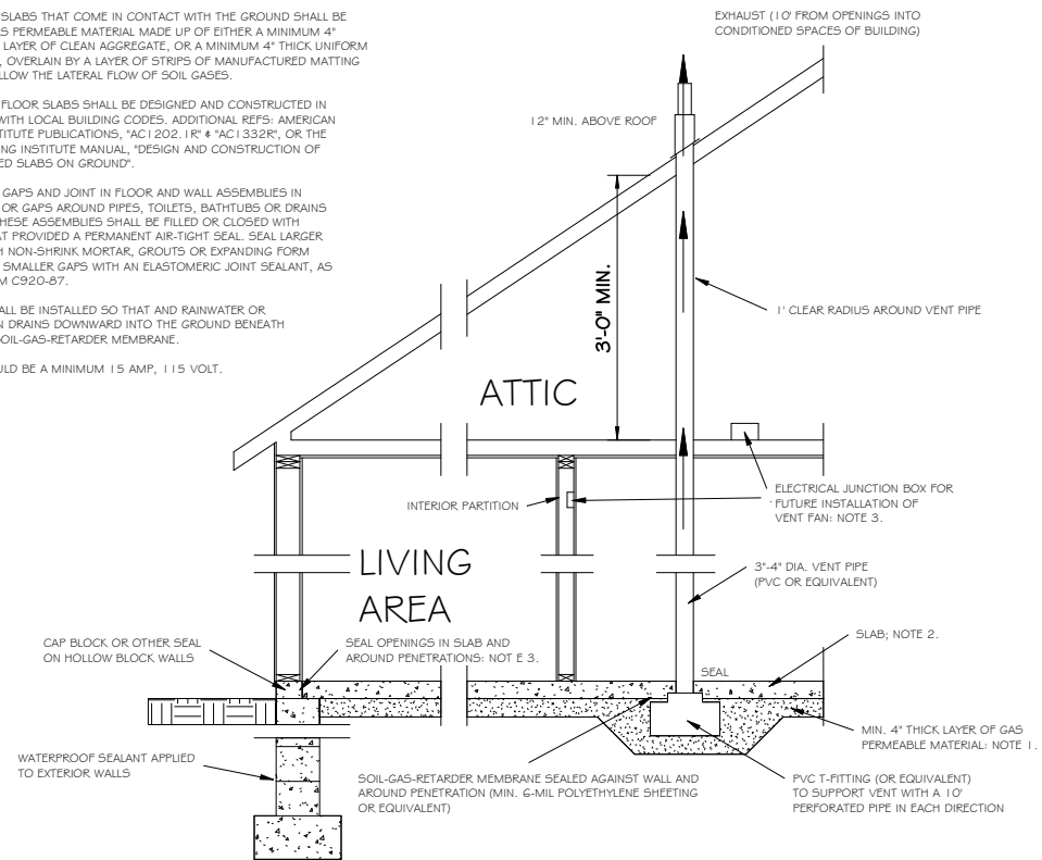
3 - Radon Section 1/2" = 1'-0"
