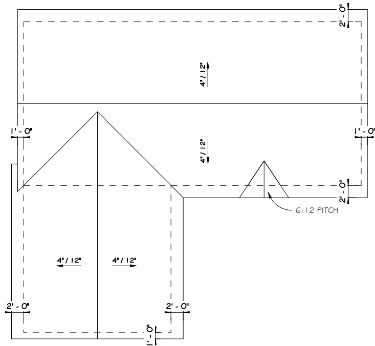
5 ROOF PLAN 1/8" = 1'-0"
