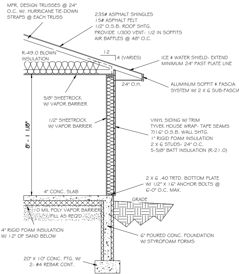
6 - Wall Section 1/2" = 1'-0"
