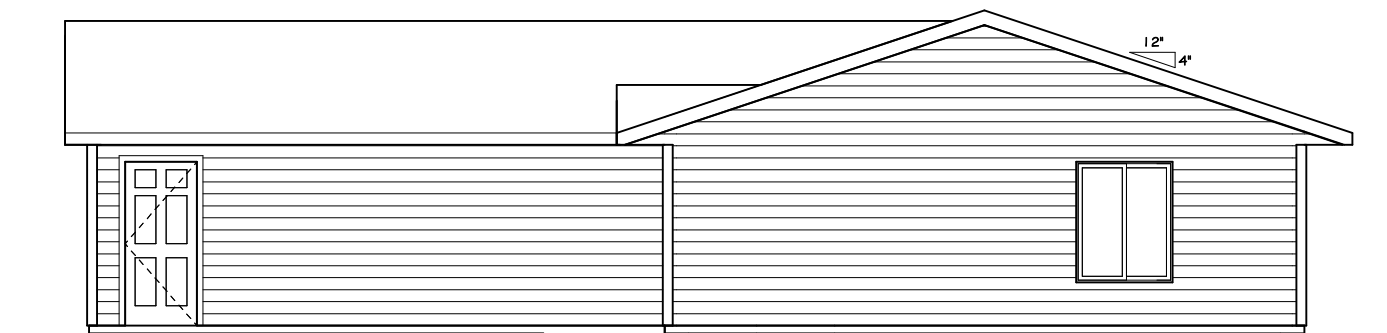
2 RIGHT 1/4" = 1'-0"
