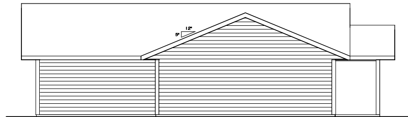
2 LEFT ELEVATION 1/4" = 1'-0"
