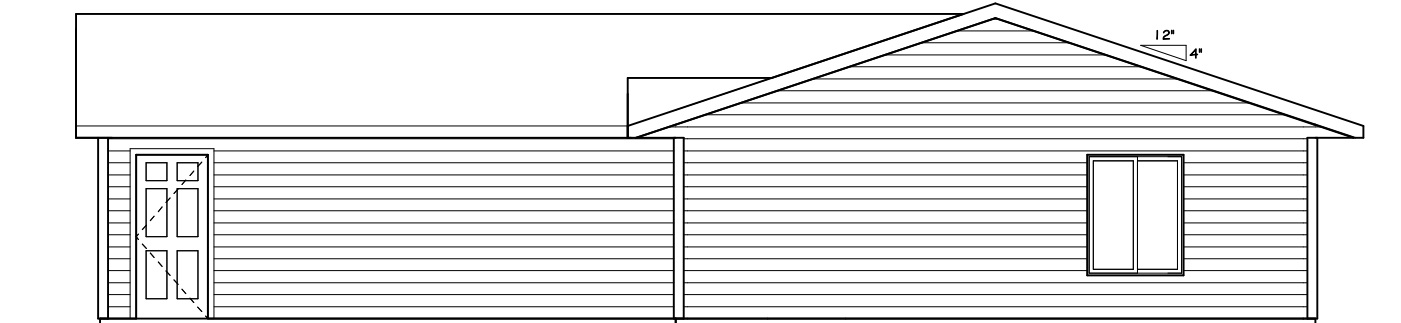
2 RIGHT 1/4" = 1'-0"
